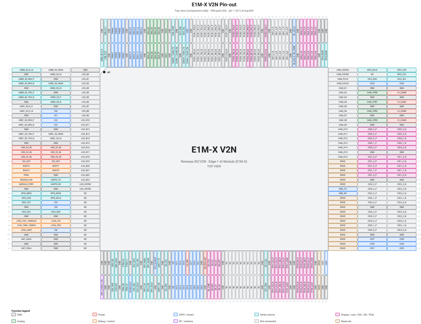
Figure 4 E1M-X V2N Pin-out (top view, 496-pad LGA)
